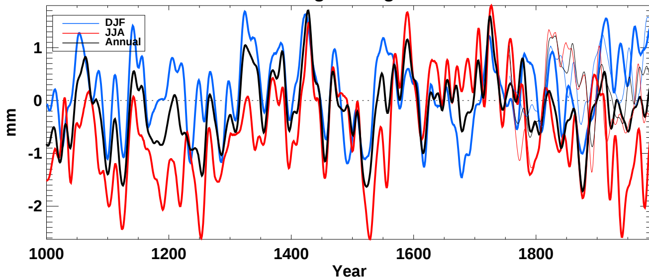
soilm from echo-g averaged over SH land
