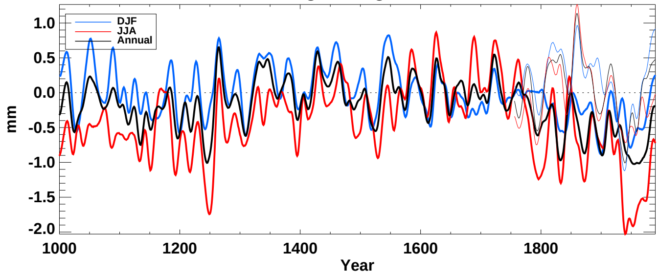
soilm from echo-g averaged over Global land
