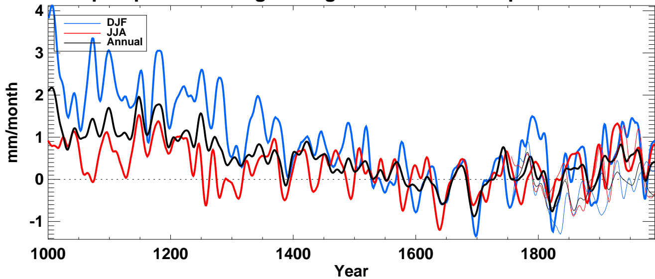
precip from echo-g averaged over N-extratropics ocean
