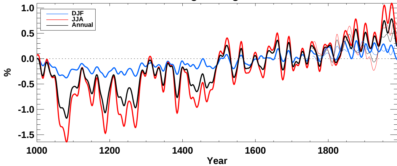
iceco from echo-g averaged over SH ocean
