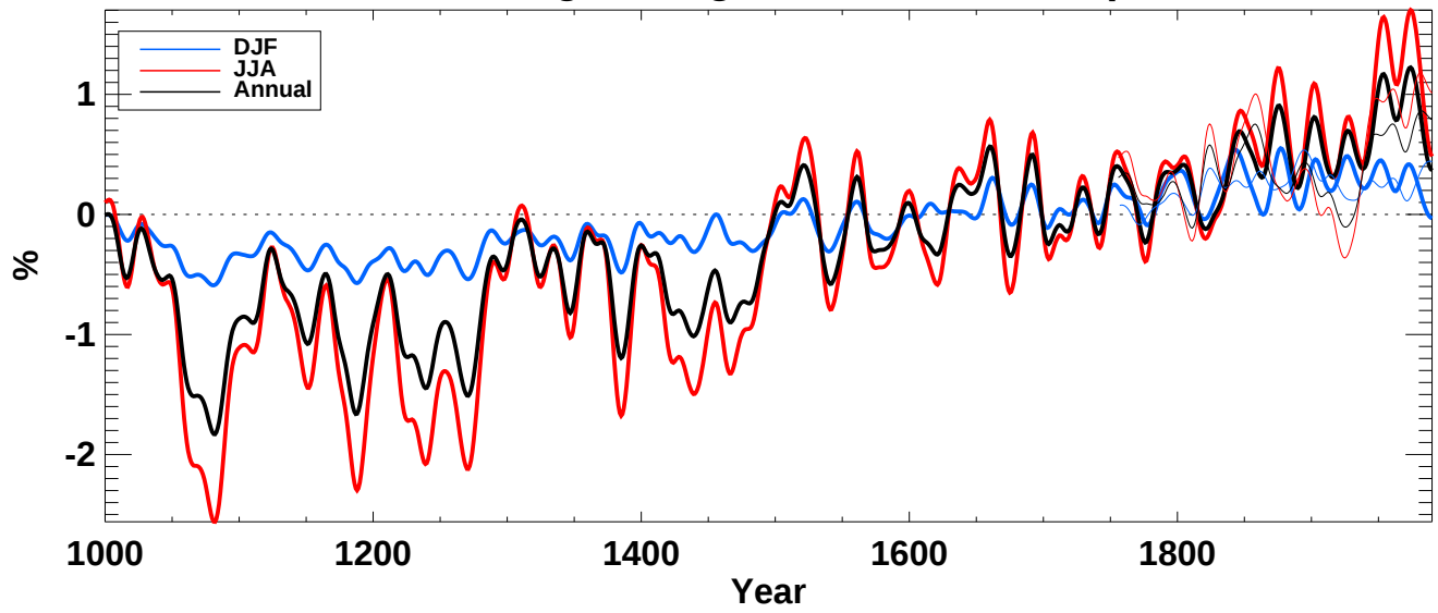
iceco from echo-g averaged over S-extratropics ocean
