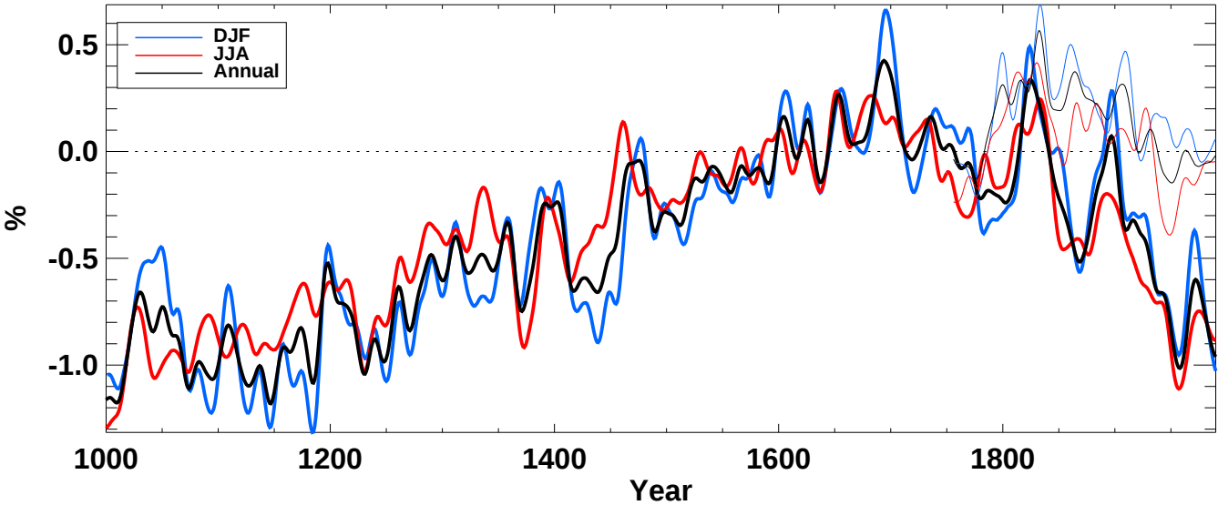
iceco from echo-g averaged over N-extratropics ocean
