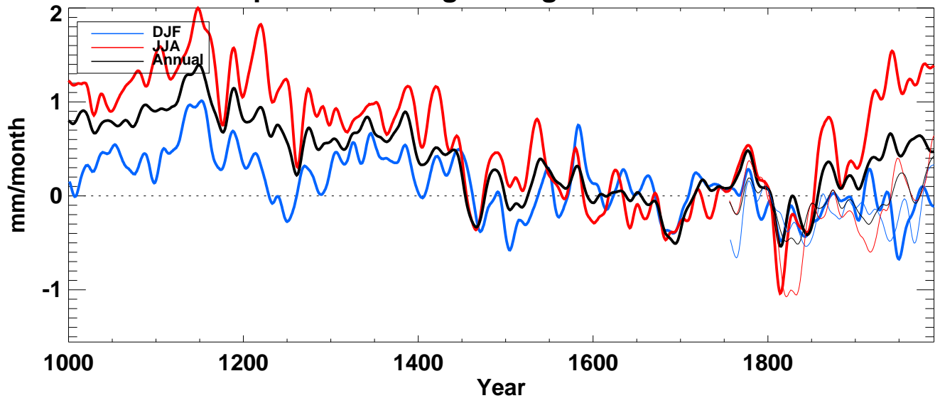
evap_ from echo-g averaged over SH ocean
