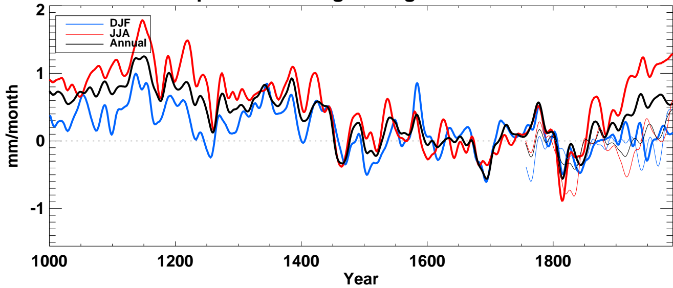
evap_ from echo-g averaged over SH full
