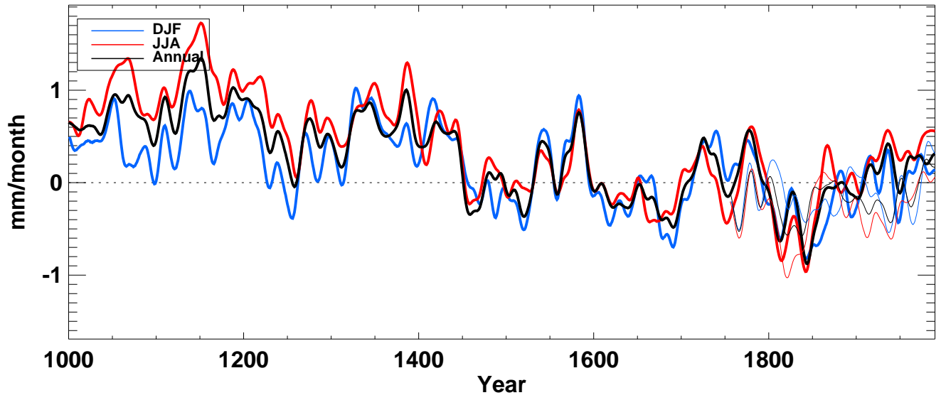
evap_ from echo-g averaged over S-extratropics full
