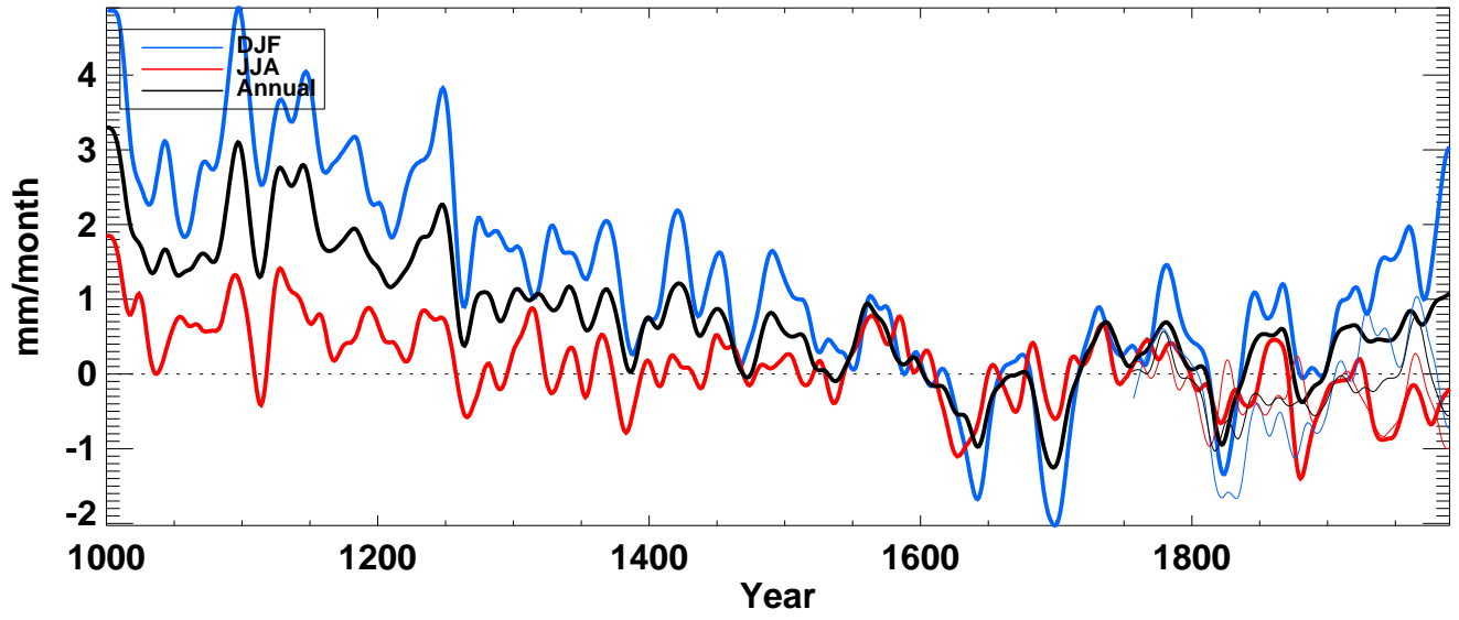
evap_ from echo-g averaged over N-extratropics ocean
