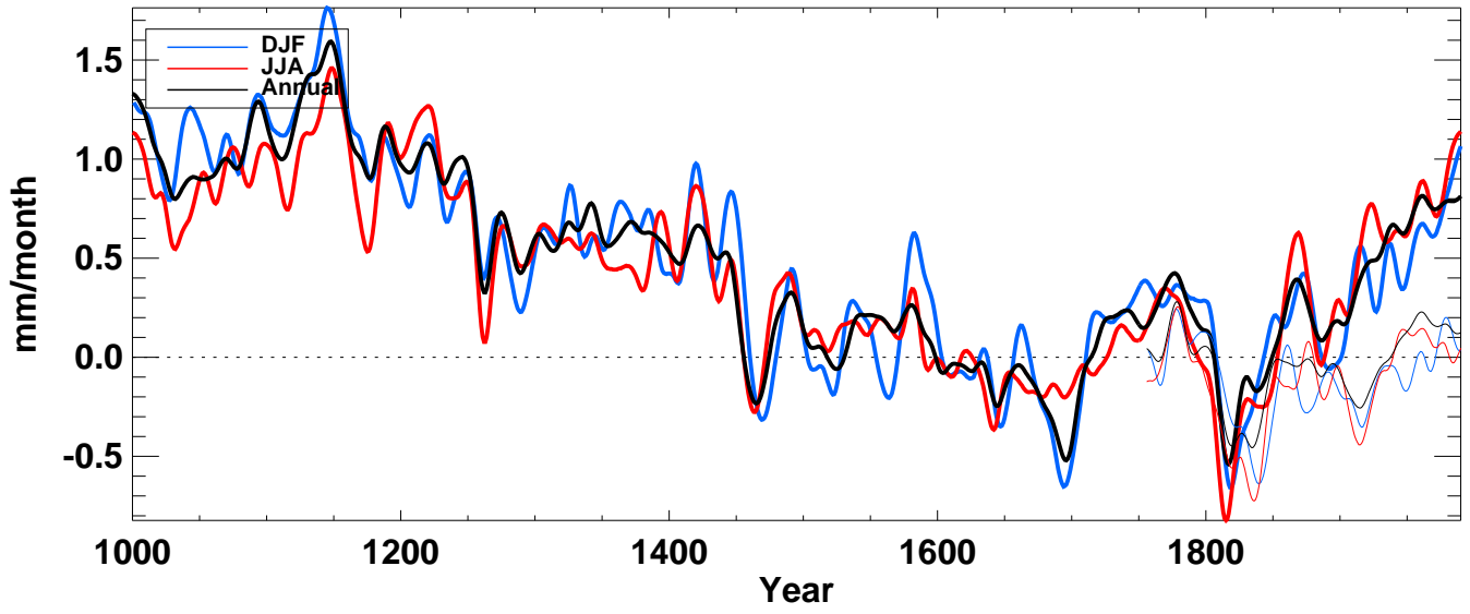
evap_ from echo-g averaged over Global ocean
