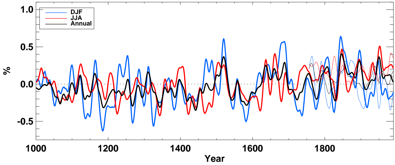
cloud from echo-g averaged over S-extratropics ocean
