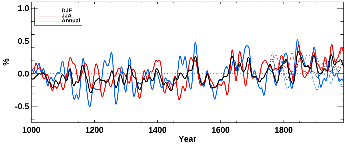
cloud from echo-g averaged over S-extratropics full
