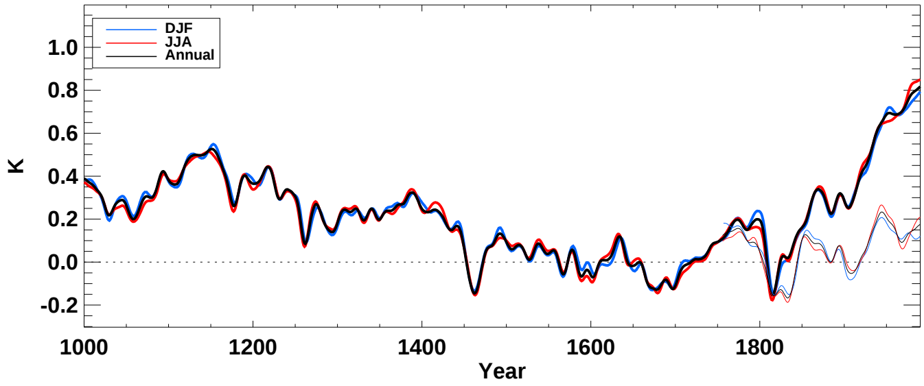
airtm from echo-g averaged over Tropics ocean
