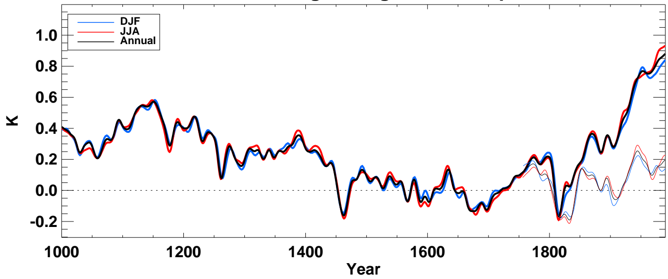
airtm from echo-g averaged over Tropics full
