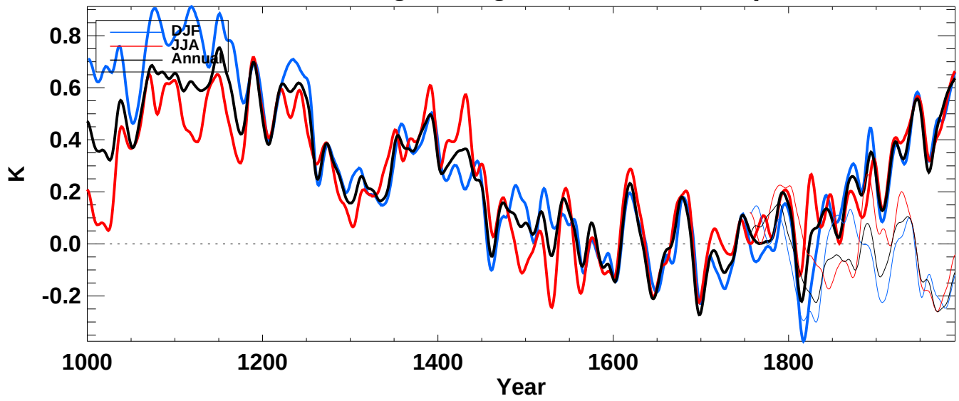
airtm from echo-g averaged over S-extratropics land
