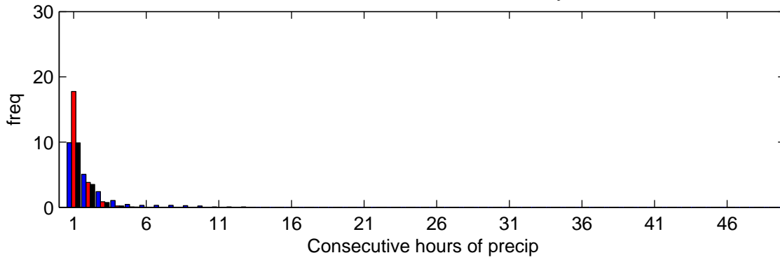
Frequency of wet hour amounts – January
