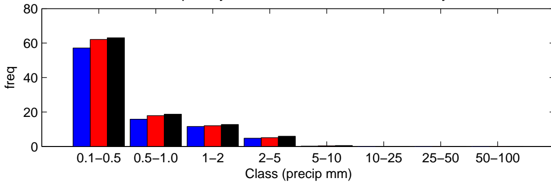
Frequency of wet hour amounts – July
