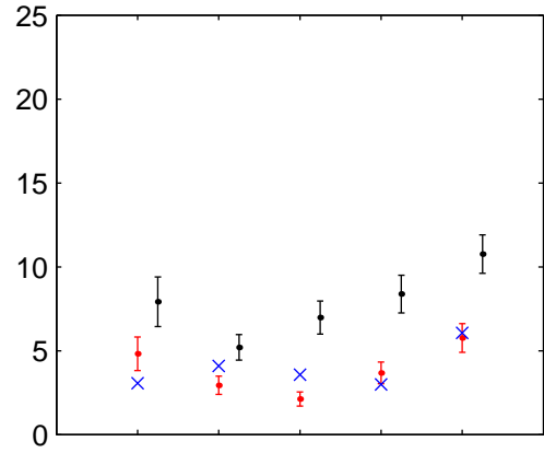
Heatwave duration
