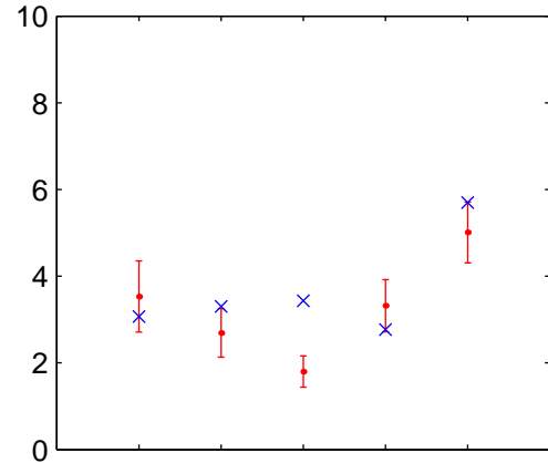
Heatwave duration
