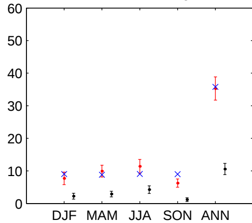
Number of "Cold nights"
