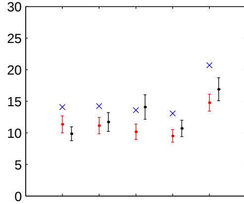
Maximum number of consecutive dry days
