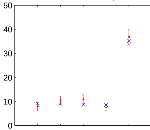
Number of "Warm nights"
