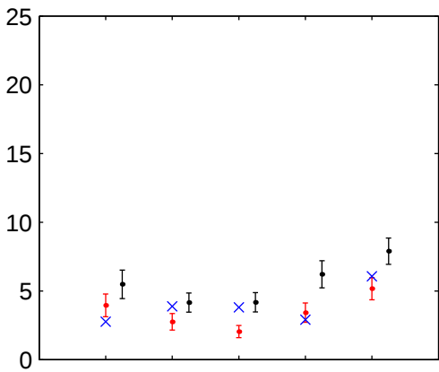
Heatwave duration
