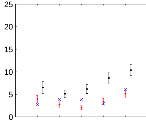
Heatwave duration
