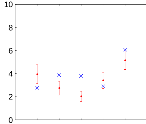
Heatwave duration
