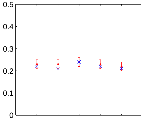
Fraction of total precipitation from intense events
