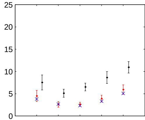
Heatwave duration
