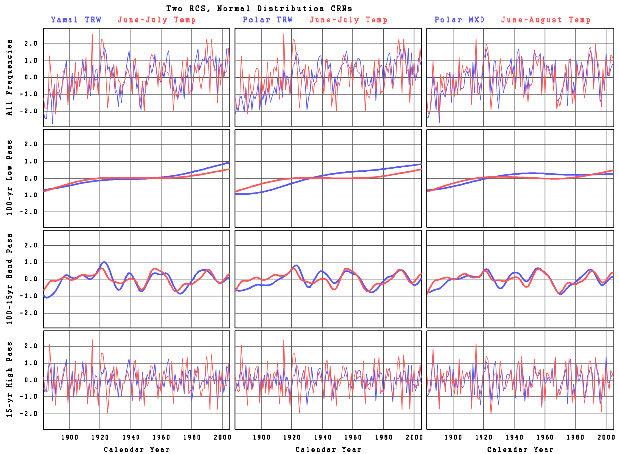
Figure CA5 Chronologies were created using processing methods as described in Figure CA3 using two-curve, signal-free RCS with tree indices transformed to have a normal distribution. Series are potted over the common period between chronologies and temperature data for each of the frequency divisions (from the top all frequencies, 100-year low-pass, 15-100-year band-pass, and 15-year high pass) and for the three separate chronologies from left to right: Yamal TRW, Polar Urals TRW and Polar Urals MXD.
