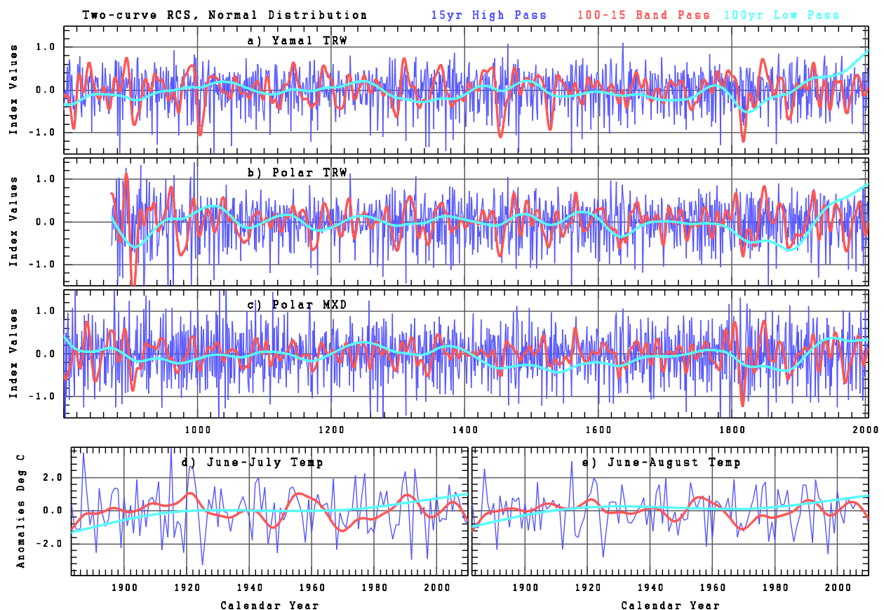
Figure CA3 Chronologies created for Yamal TRW (a), Polar Urals TRW (b) and Polar Urals MXD (c) using two curve signal-free RCS and tree indices converted to have a Normal distribution. These chronologies were separated into 15-year high-pass, 15-100-year band-pass, and 100-year low-pass chronologies using smoothing splines. Because the indices are approximately normally distributed in these chronologies, the signals were separated using subtraction; as a result the sum of the high-pass, band-pass and low-pass chronologies will be the full chronology. The adjusted CRUTEM4v temperature series for 67.5N, 67.5E (mean of June and July (d) for TRW and mean of June to August (e) for MXD) were also separated into 15-year high-pass, 15-100-year band-pass, and 100-year low-pass chronologies using smoothing splines, with separation by subtraction; the sum of the high-pass, band-pass and low-pass temperature series reconstitutes the “full” observed temperature series.
