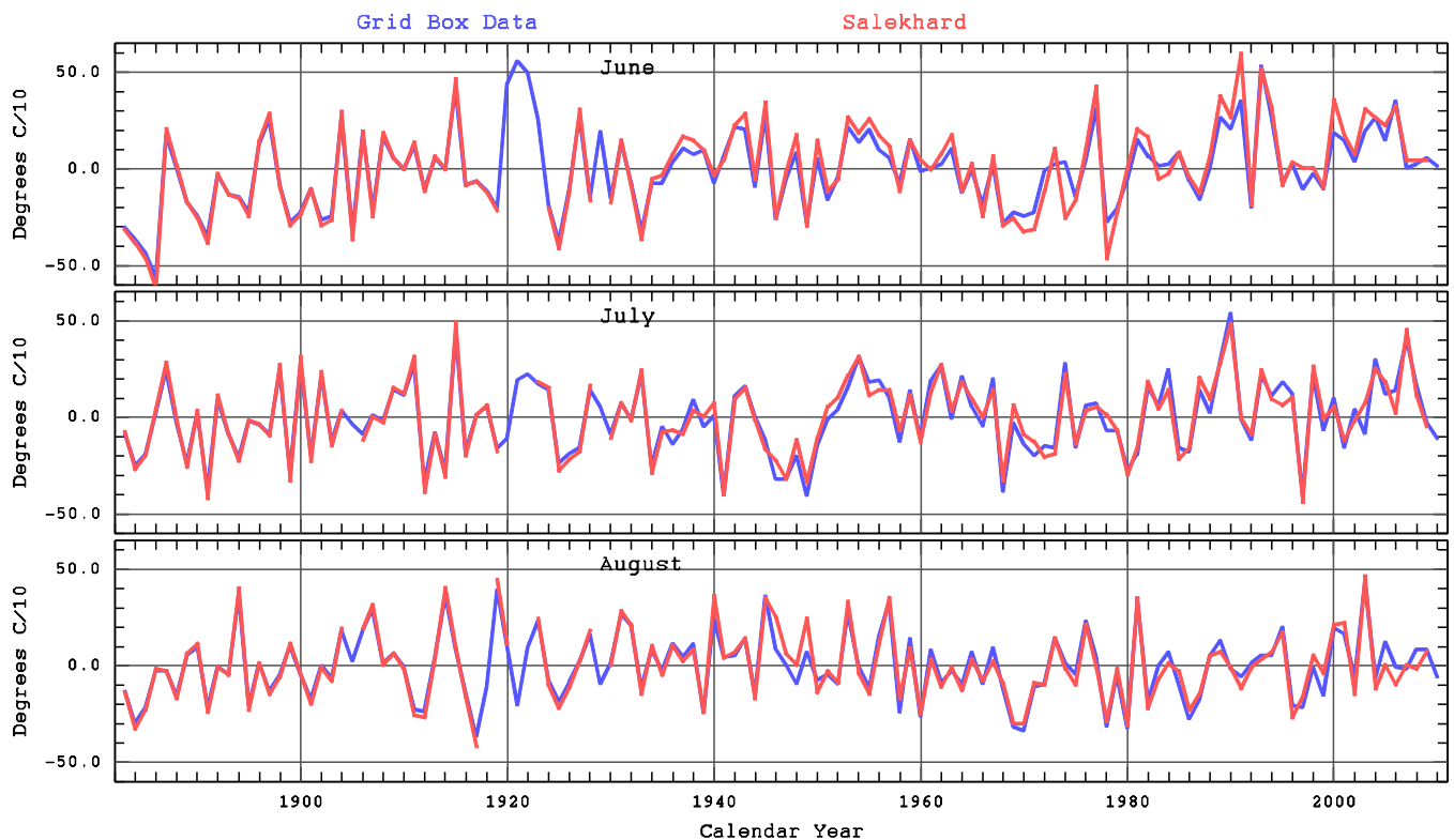
Figure CA1 Monthly temperature series showing in-filled values (blue).
