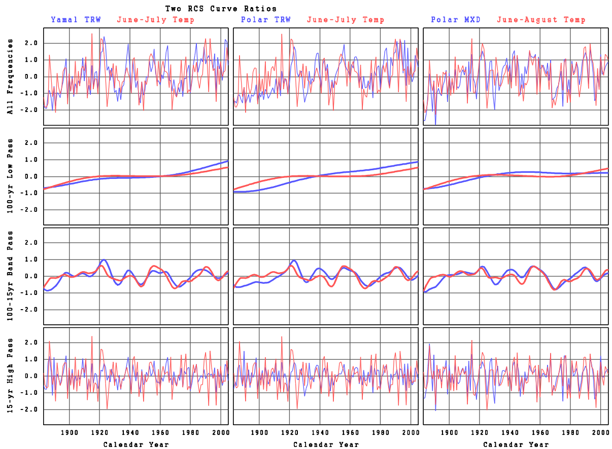
Figure CA4 Chronologies were created using processing methods as described in Figure CA2 using two-curve, signal-free RCS which produces tree indices as ratios and compared with temperature data. Series are plotted over the common period between chronologies and temperature data for different frequency divisions (from the top all frequencies, 100-year low-pass, 15-100-year band-pass, and 15-year high pass) and for the three separate chronologies from left to right: Yamal TRW, Polar Urals TRW and Polar Urals MXD.
