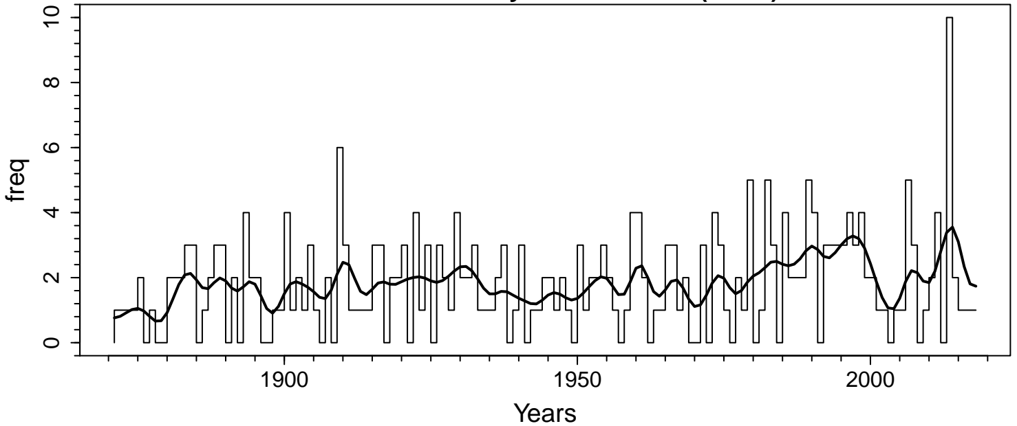
UK NDJFMA Very Severe Gales (G>50)
