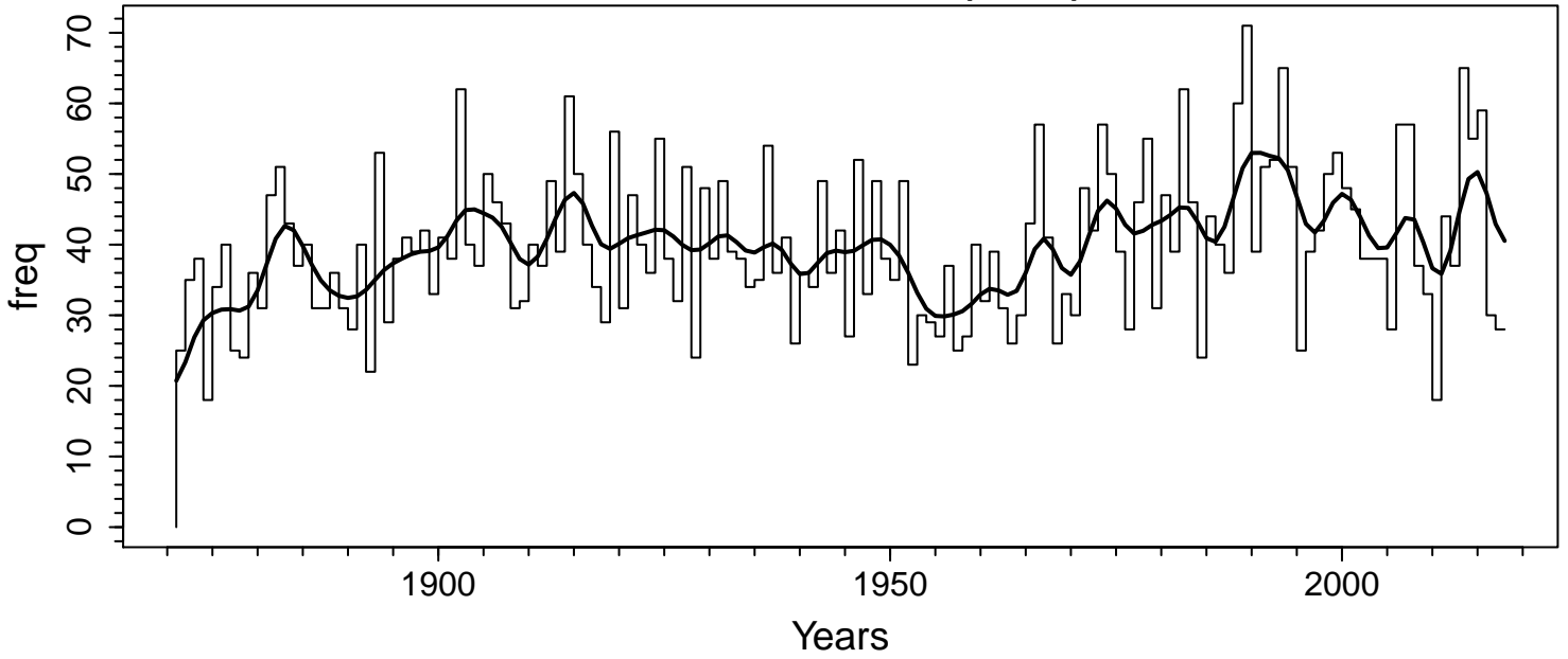
UK NDJFMA Severe Gales (G>40)
