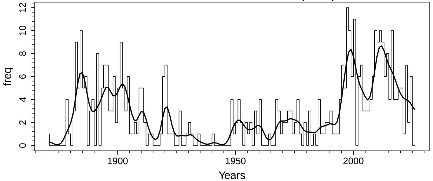
Falklands MJJASO Very Severe Gales (G>25)
