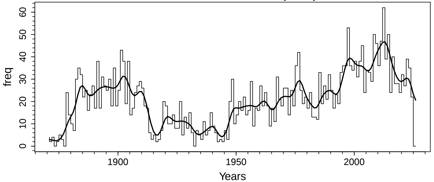
Falklands MJJASO Severe Gales (G>20)
