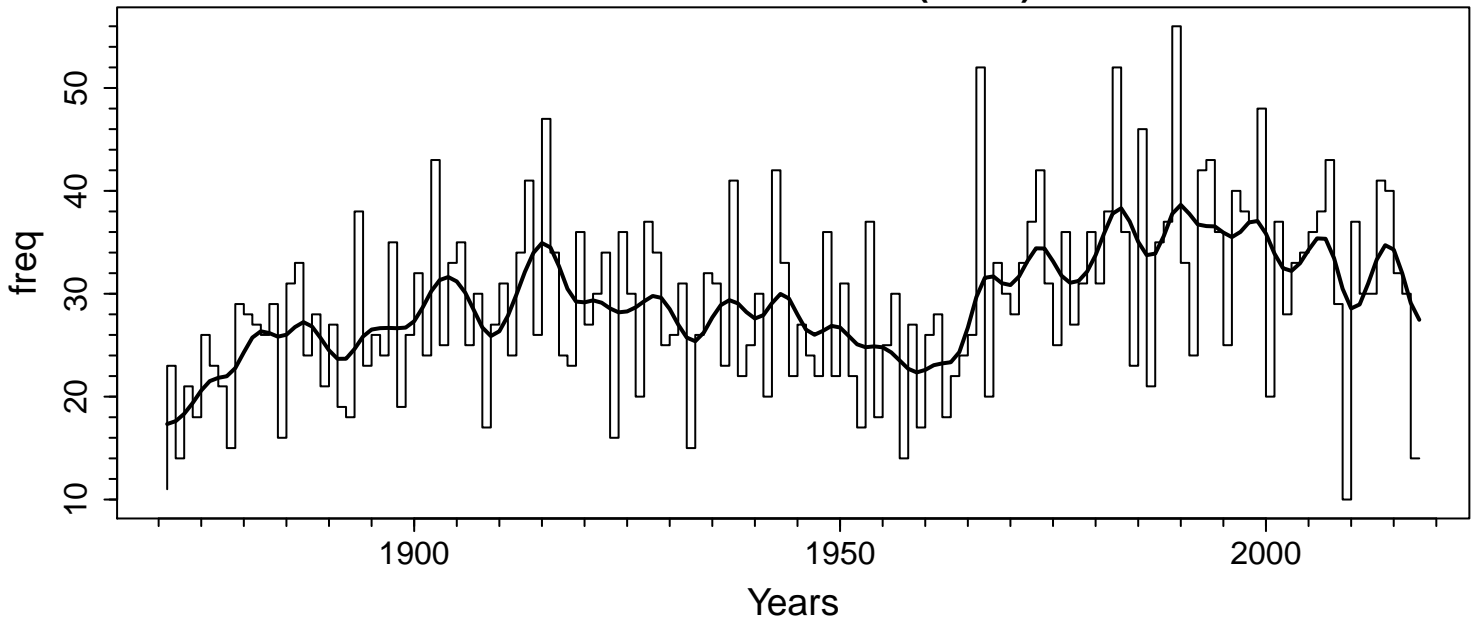
N Sea Annual Severe Gales (G>40)
