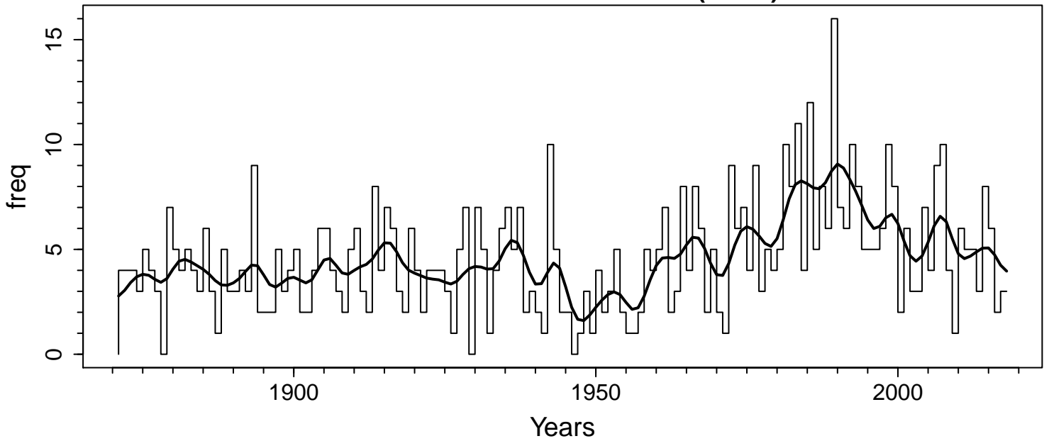
N Sea Annual Very Severe Gales (G>50)
