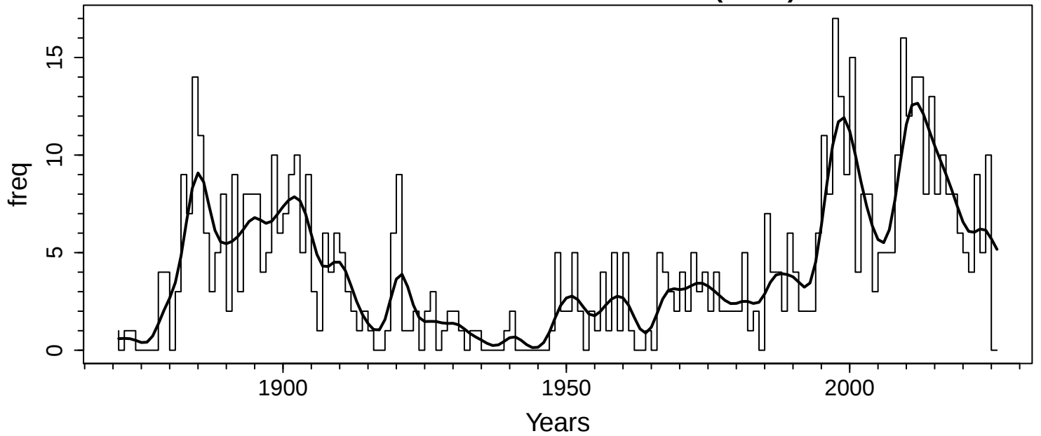
Falklands Annual Very Severe Gales (G>25)
