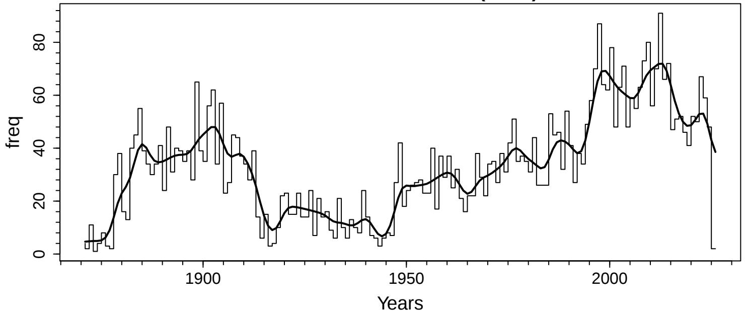
Falklands Annual Severe Gales (G>20)
